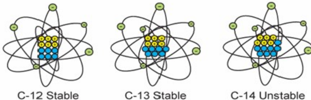
stable & unstable atoms (figure 1)
